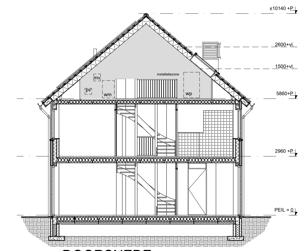
DOORSNED E
